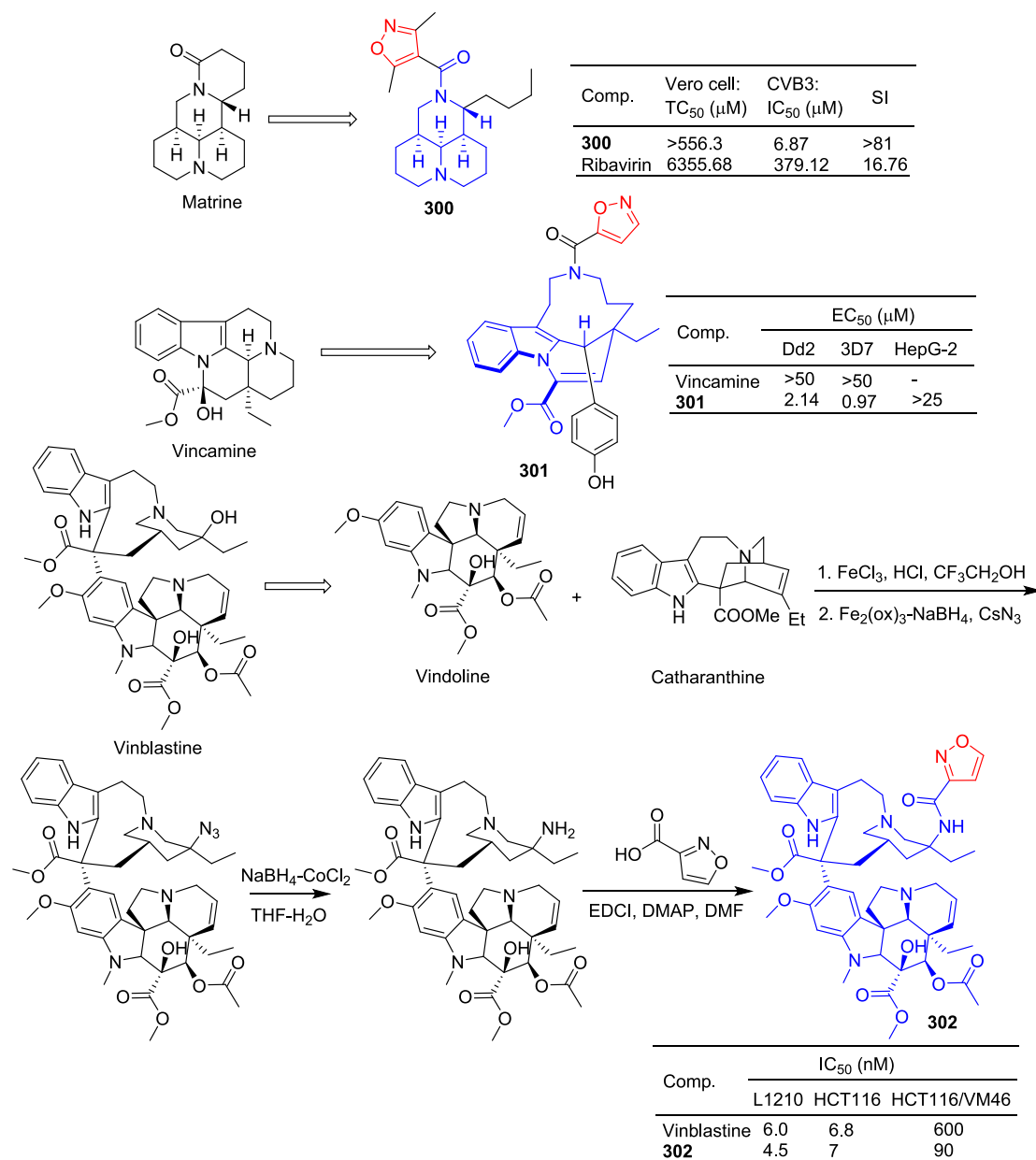
Fig. 66. Alkaloid-isoxazole derivatives 300–302.
