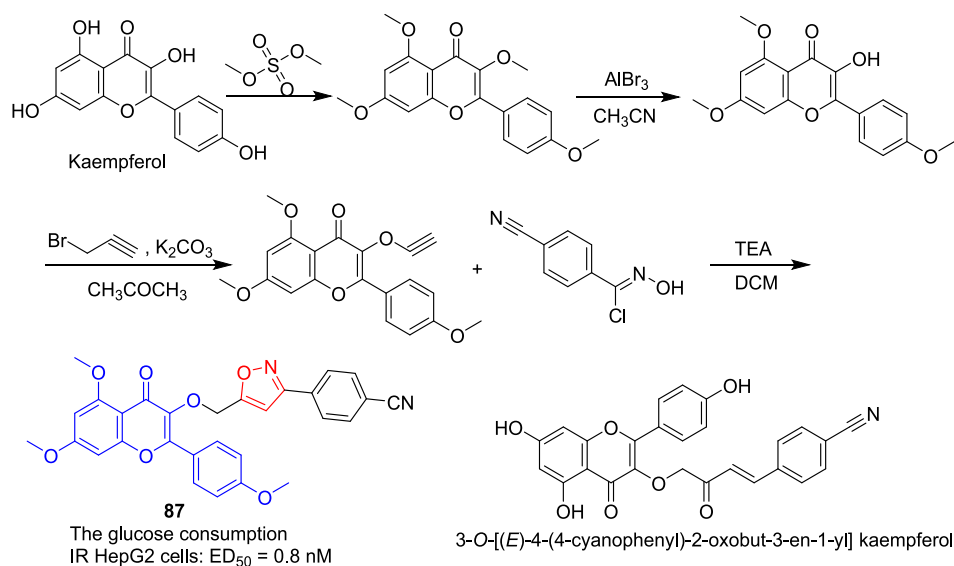
Fig. 24. Flavono-isoxazole derivative 87 .
