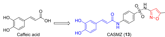
Fig. 5. Cinnamamide-isoxazole derivatives 6–13.
