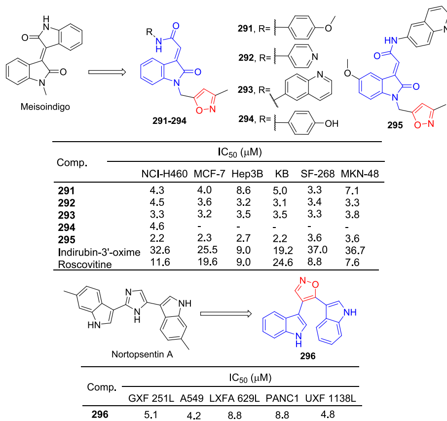
Fig. 64. Alkaloid-isoxazole derivatives 291–296.
