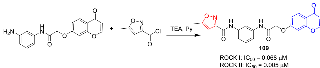
Fig. 28. Chromone-isoxazole derivatives 103–109 .
