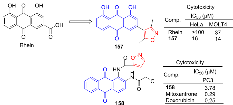
Fig. 38. Anthraquinone-isoxazole derivatives 157–158.
