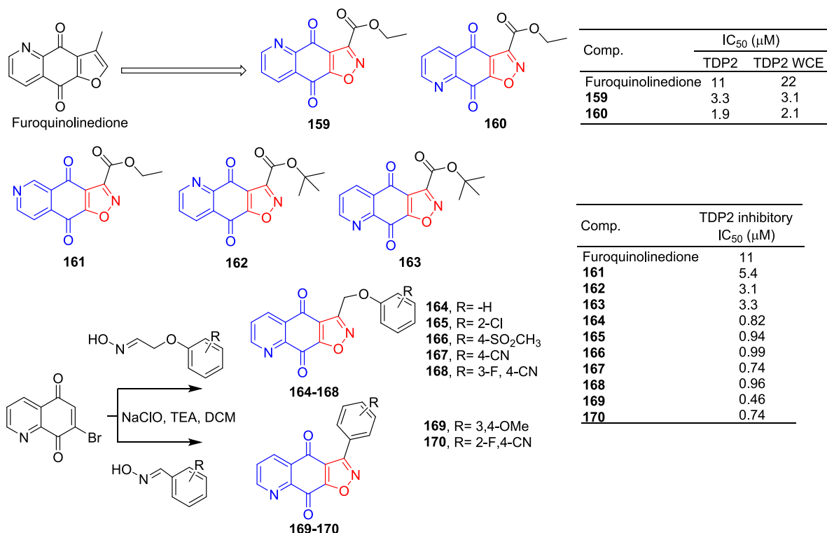
Fig. 39. Naphthoquinone-isoxazole derivatives 159–170.
