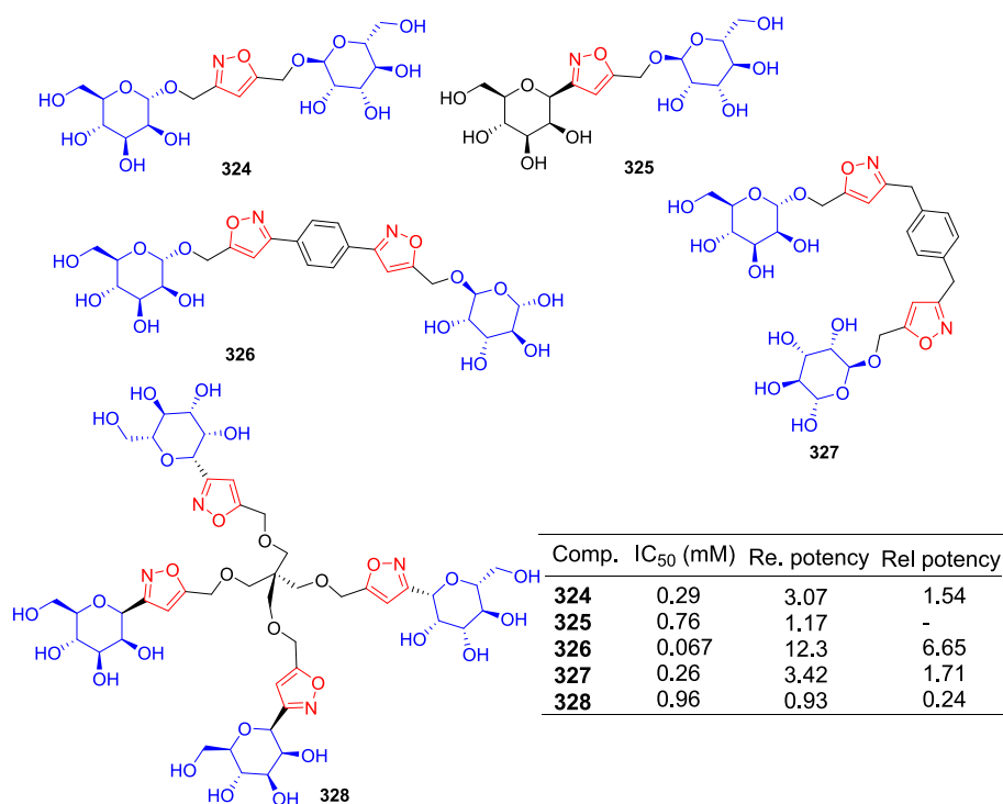
Fig. 72. Carbohydrate-isoxazole derivatives 324–328.
