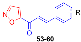
53 , R= 2,4-OCH 3 54 , R= 2,4,6-OCH 3 55 , R= 2-Cl, 4,6-OCH 3 56 , R= 2,3,4-OCH 3 57 , R= 2,4,5-OCH 3 58 , R= 3,4,5-OCH 3 59 , R= 3,4-OCH 3 60 , R= 2-F, 3,4-OCH 3
