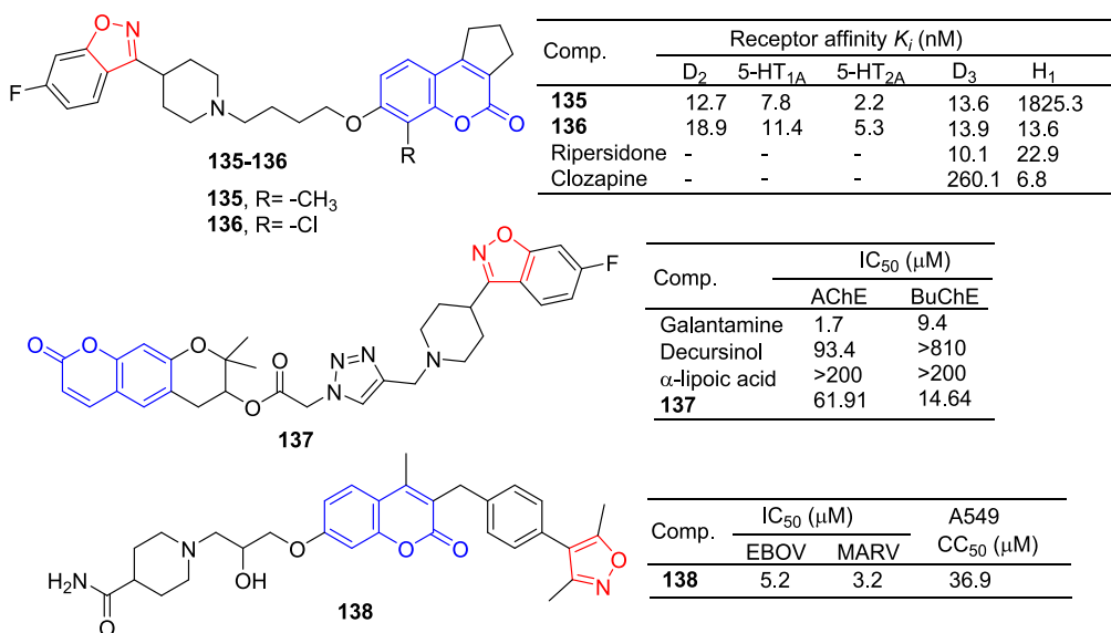
Fig. 33. Coumarin-isoxazole derivatives 130–138.
