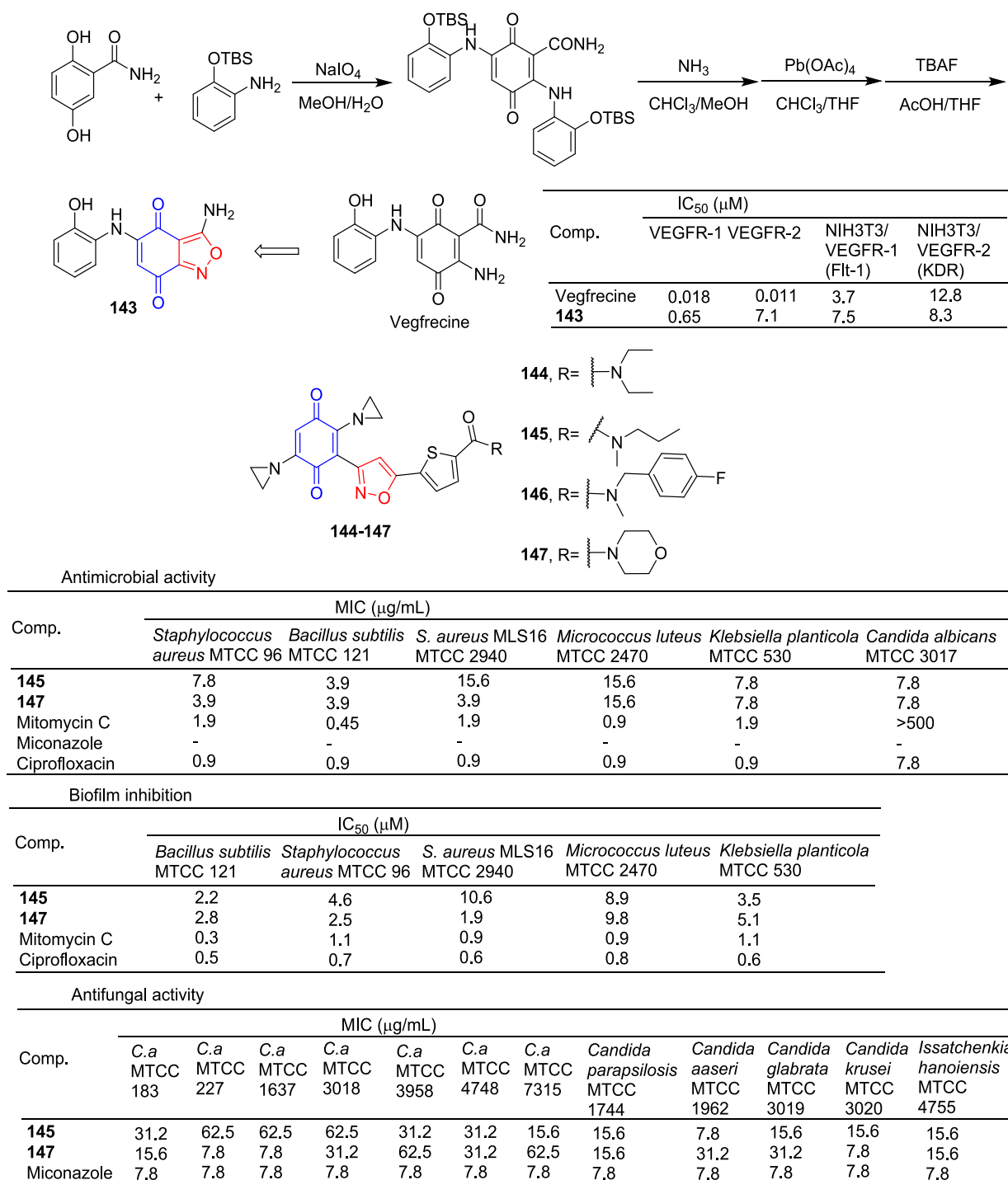
Fig. 35. Benzoquinone-isoxazole derivatives 143–147.
