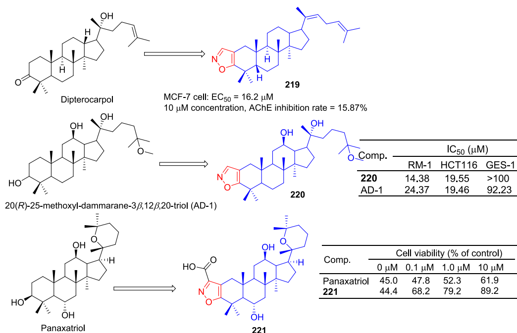
Fig. 48. Steroidal-isoxazole derivatives 219–221.
