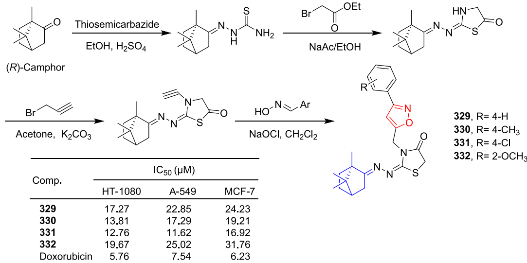
Fig. 73. Camphor-isoxazole derivatives 329 – 332 .
