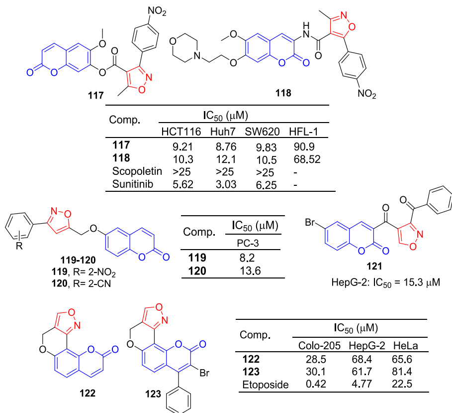
Fig. 30. Coumarin-isoxazole derivatives 117 – 123 .
