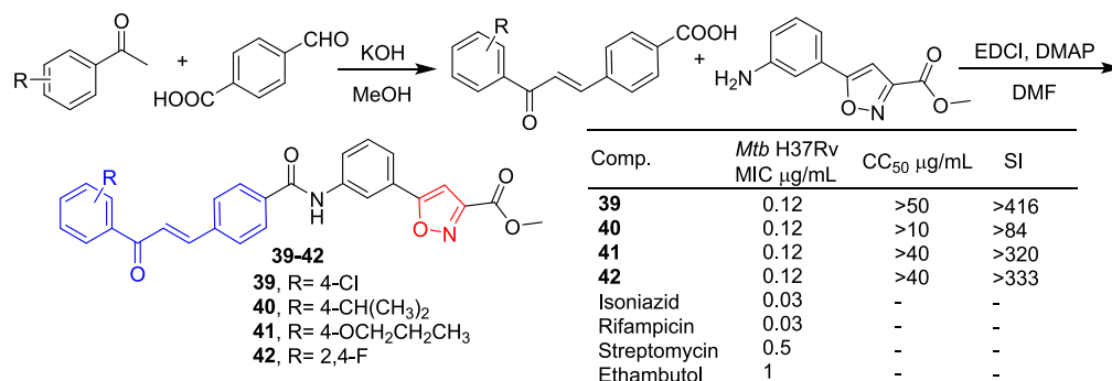
Fig. 11. Chalcone-isoxazole derivatives 39–42.
