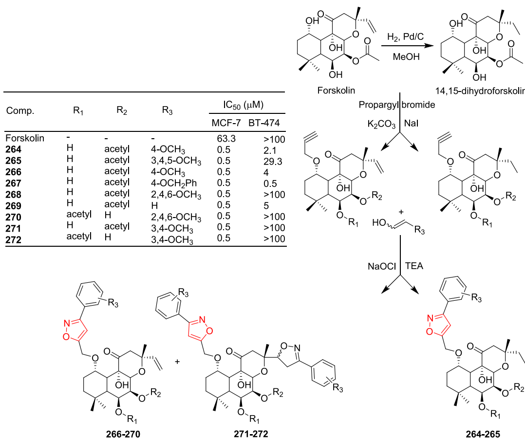
Fig. 56. Terpene-isoxazole derivatives 264–272.
