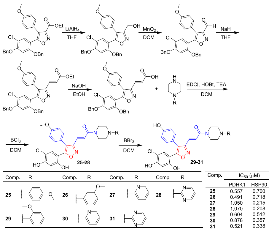
Fig. 8. Cinnamamide-isoxazole derivatives 25–31 .
