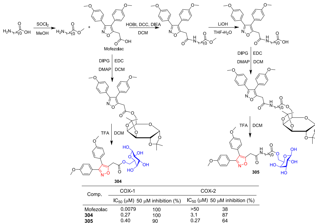
Fig. 68. Carbohydrate-isoxazole derivatives 304–305.
