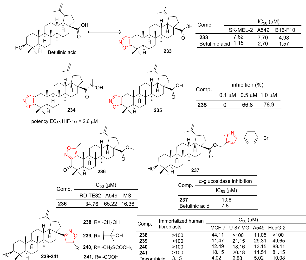
Fig. 50. Pentacyclic triterpenoids-isoazole derivatives 233–241.
