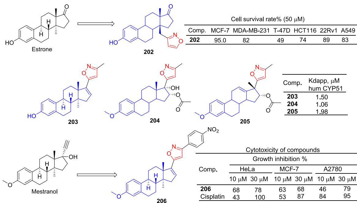
Fig. 43. Steroidal-isoxazole derivatives 202–206 .
