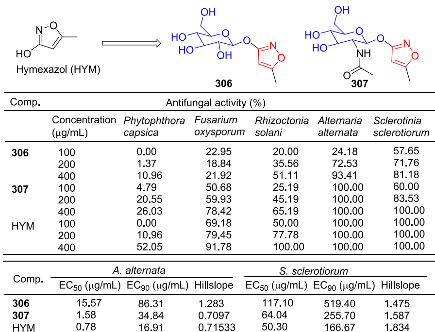
Fig. 69. Carbohydrate-isoxazole derivatives 306–307.
