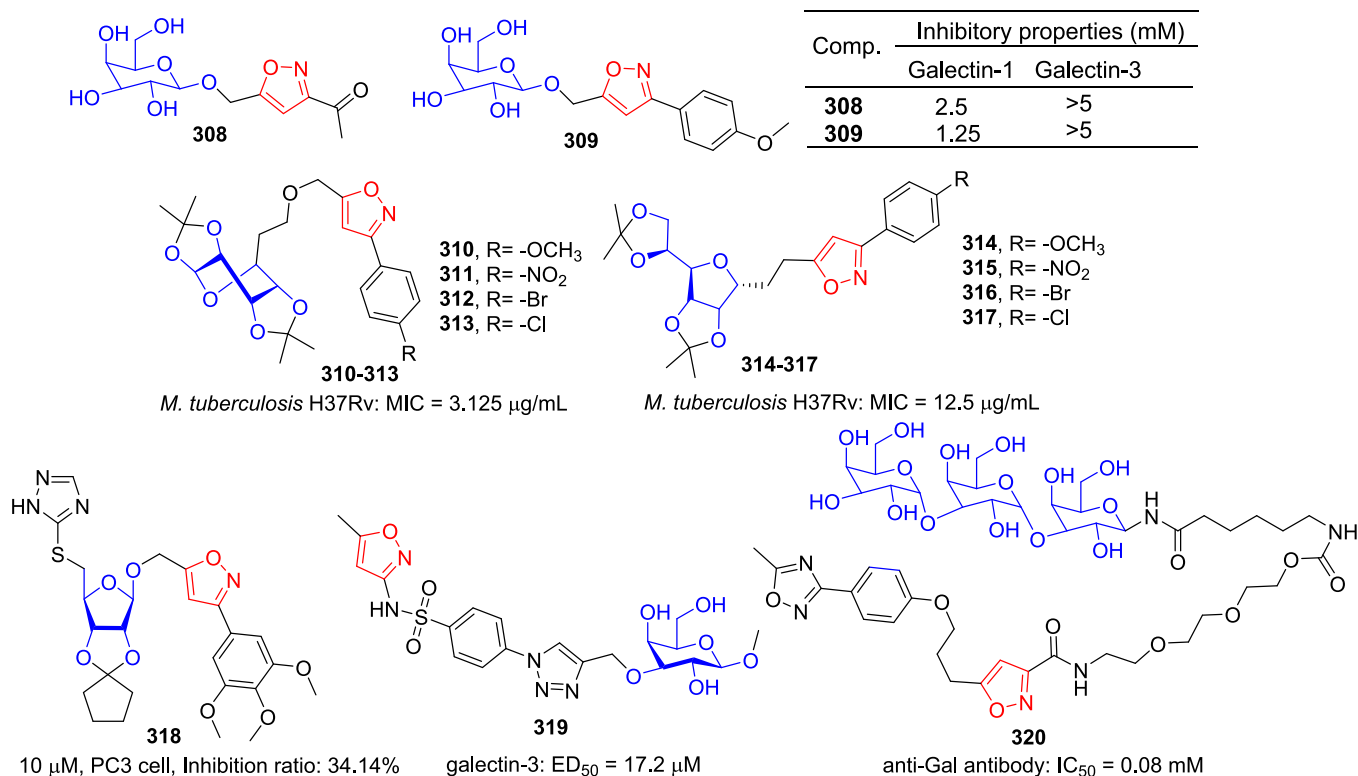
Fig. 70. Carbohydrate-isoxazole derivatives 308–320.
