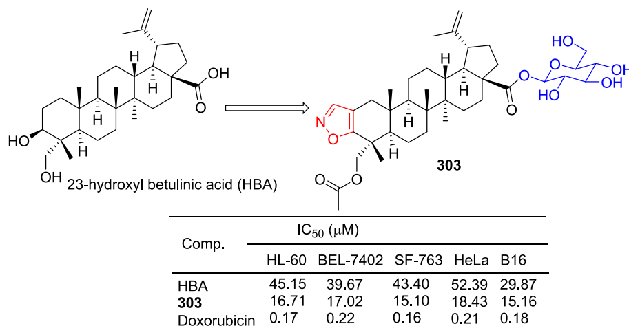
Fig. 67. Carbohydrate-isoxazole derivative 303.
