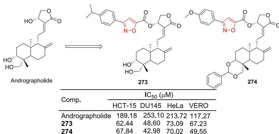
Fig. 57. Terpene-isoxazole derivatives 273–274.
