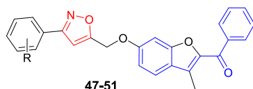
47-51 47 , R= 3-NO 2 48 , R= 4-NO 2 49 , R= 4-OCH 3 50 , R= 3,4-OCH 3 51 , R= 3-OCH 3
