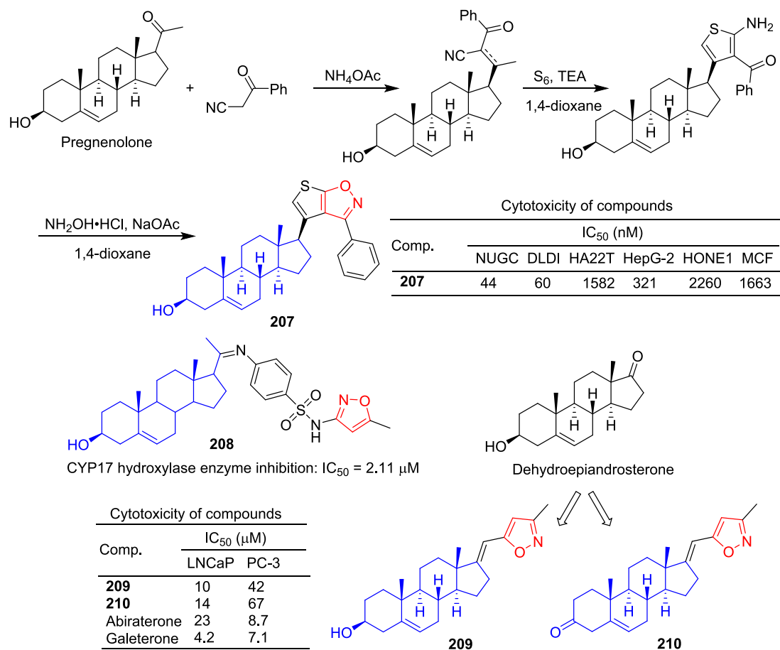
Fig. 44. Steroidal-isoxazole derivatives 207–210.
