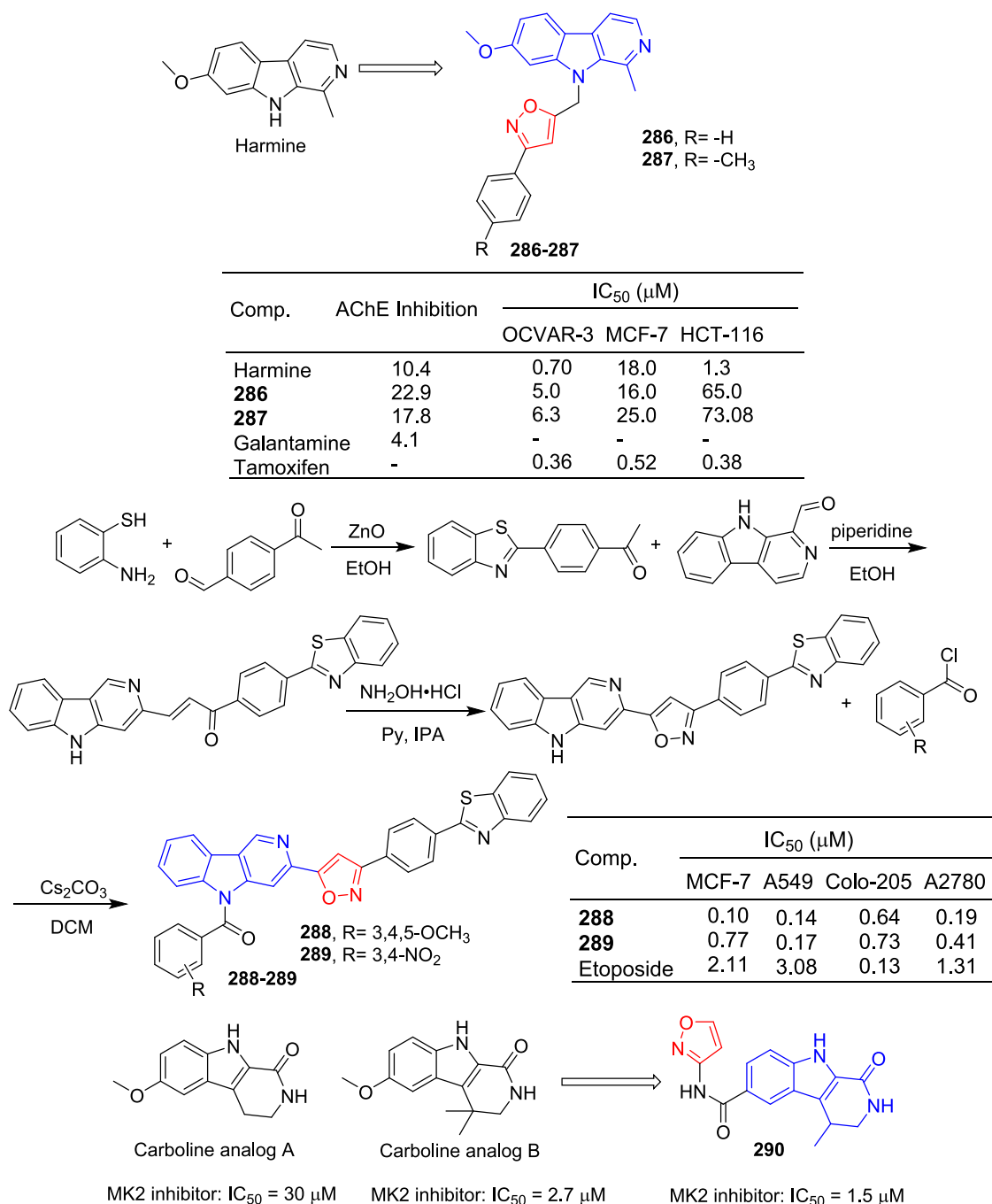
Fig. 63. Alkaloid-isoxazole derivatives 286–290 .
