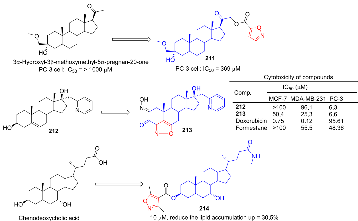
Fig. 45. Steroidal-isoxazole derivatives 211 and 213–214.
