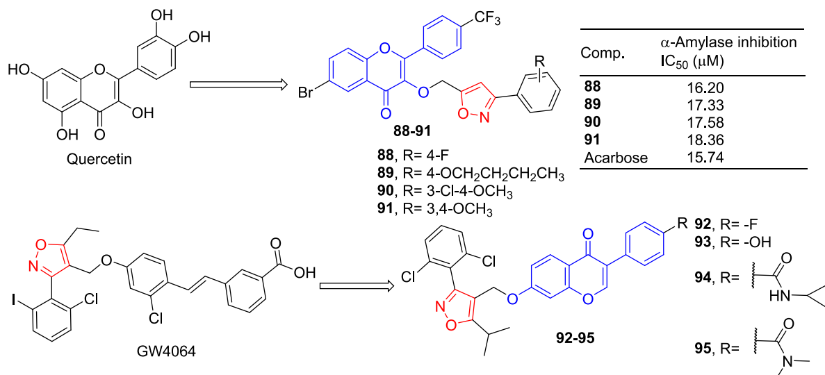
Fig. 25. Flavono-isoxazole derivatives 88–95.
