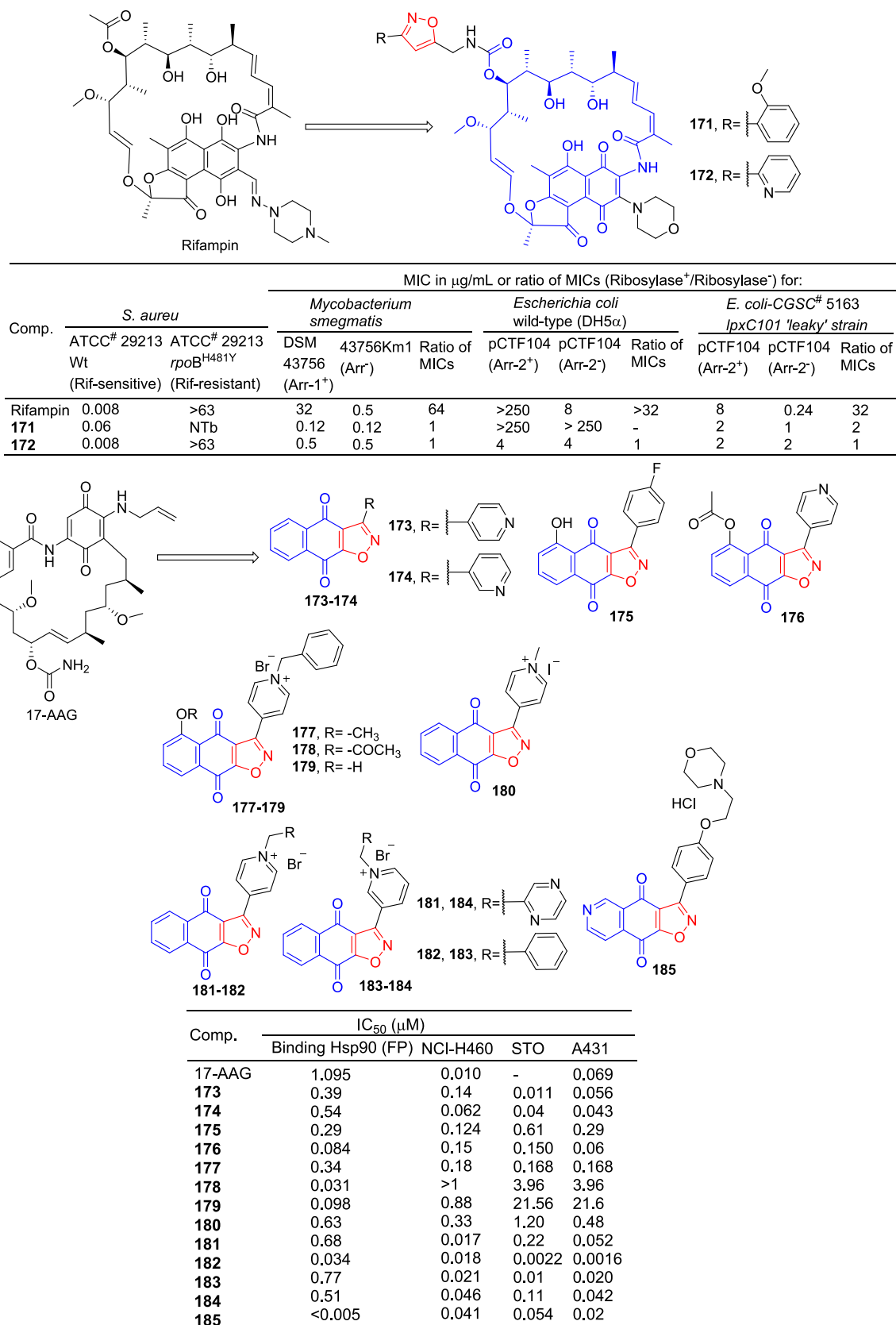
Fig. 40. Naphthoquinone-isoxazole derivatives 171–185.
