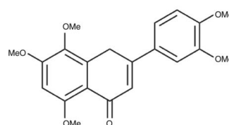
Figure 1. Structure of isosinensetin.
